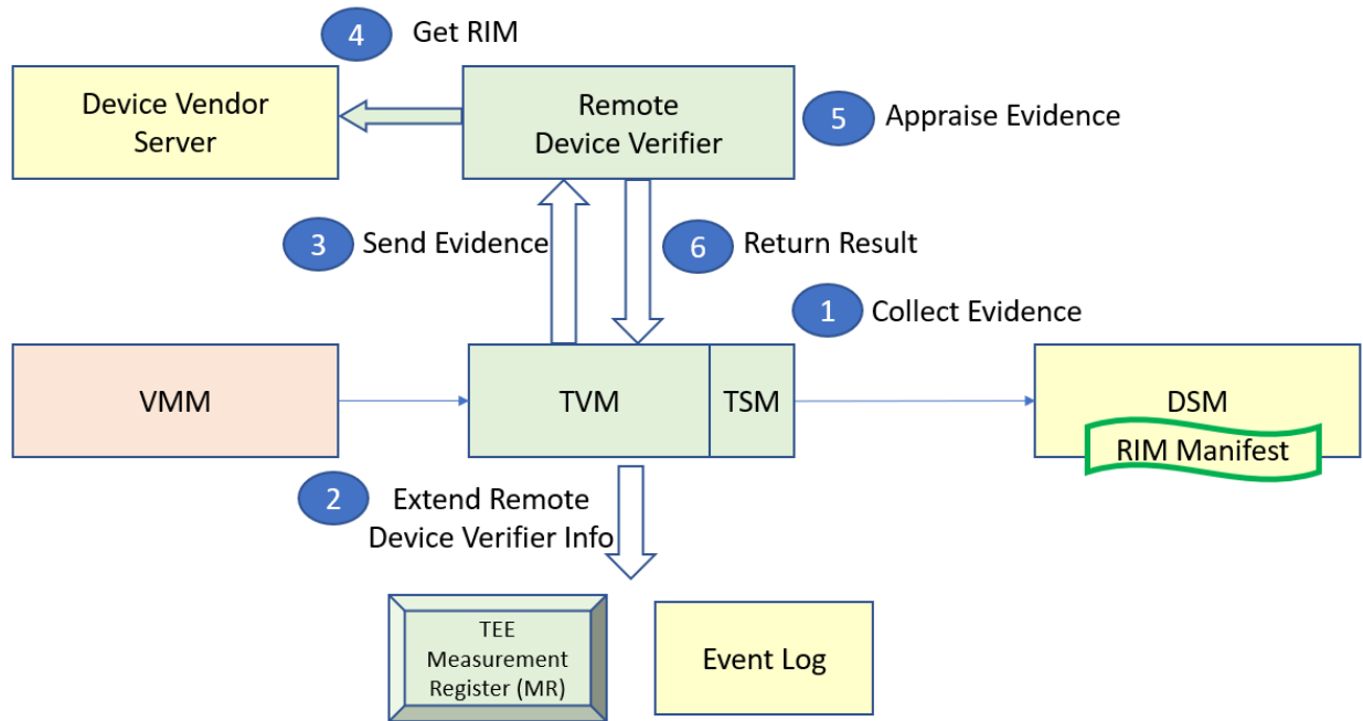
Figure 2-6: Device Remote Attestation Flow - Background Check Model
