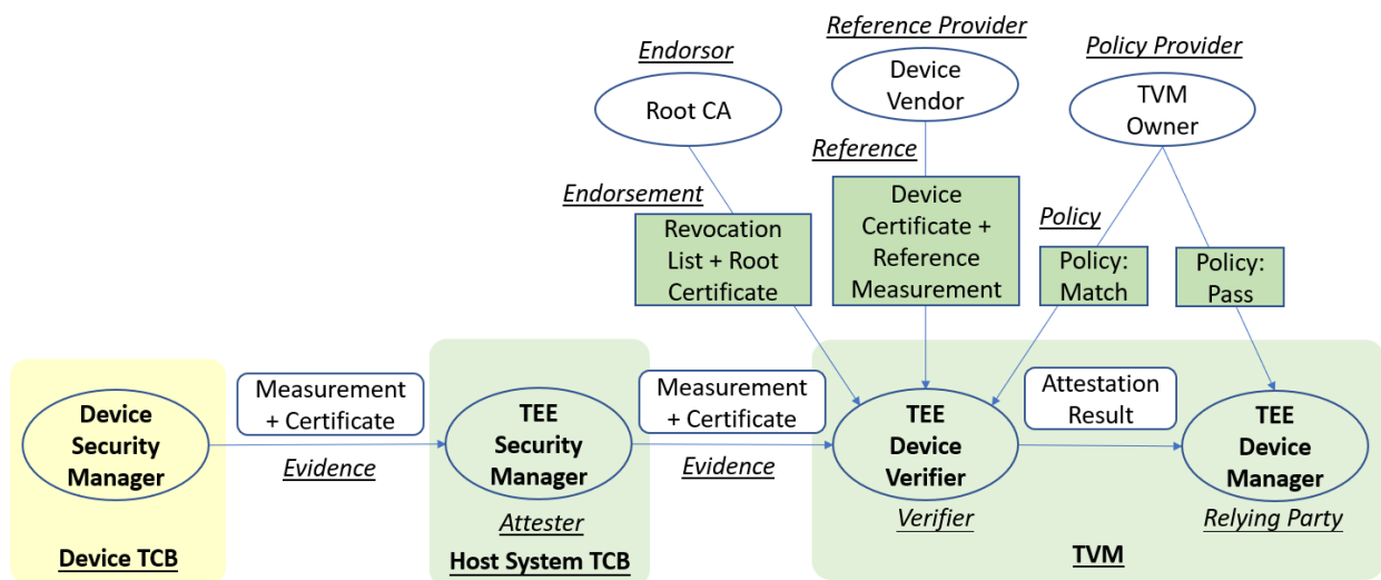
Figure 2-1: Device Local Attestation Model
