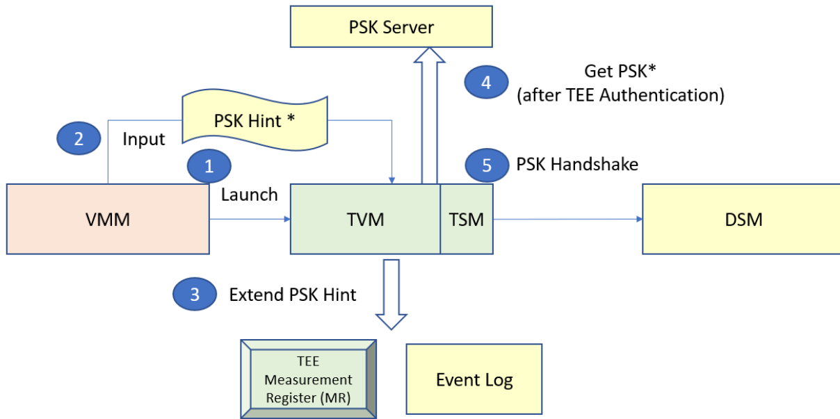
Figure 2-3: PSK based Authentication and Attestation Flow
