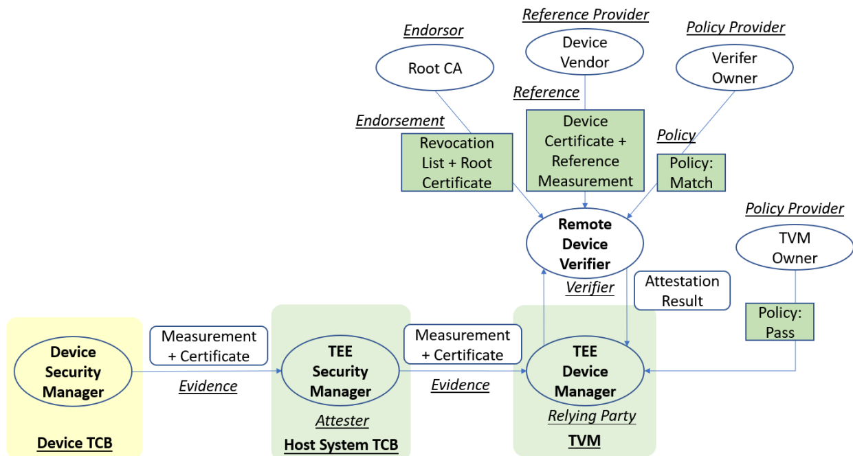
Figure 2-5: Device Remote Attestation Background Check Model
