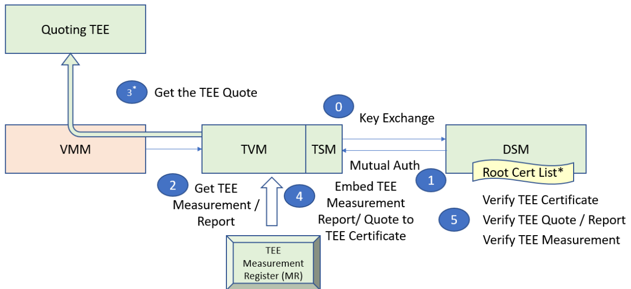
Figure 4-1: TEE Authentication
