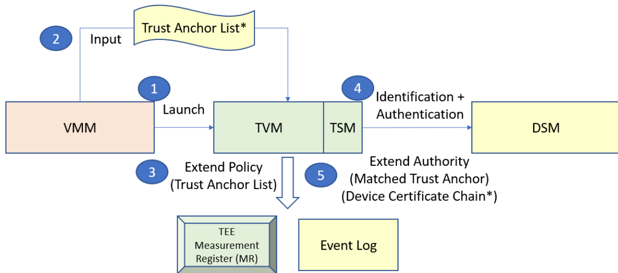
Figure 2-2: Device Authentication Flow
