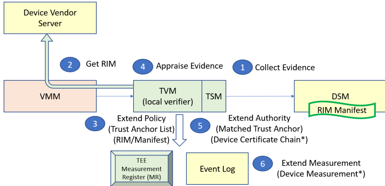
Figure 2-4: Device Local Attestation Flow
