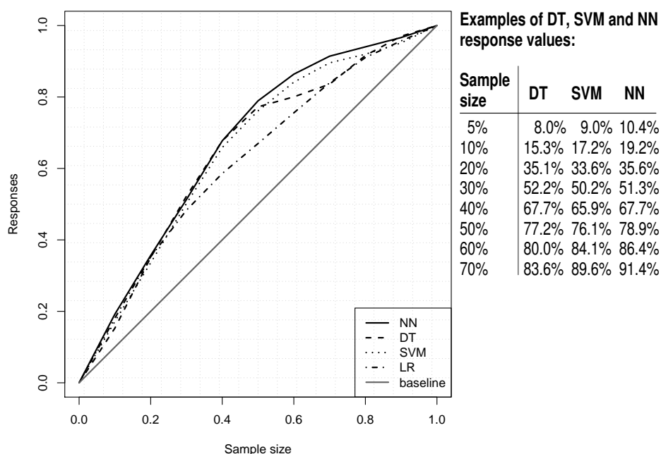
Fig. 3. Lift cumulative curves for the four models (left) and examples of NN and DT cumulative lift response values (right)
