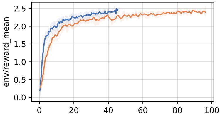
sentiment-analysis:lvwerra/distilbert-imdb
