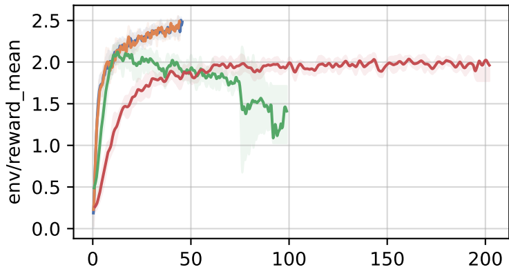
sentiment-analysis:lvwerra/distilbert-imdb
