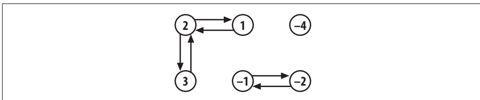
Figure 4-1. The set {1, 2, 3, -1, -2, -4} graphed according to the code block that checks adjacency
