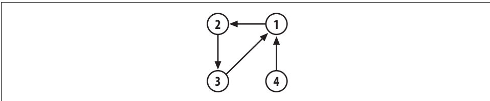
Figure 4-2. The set {1,2,3,4} graphed according to the connection hash
