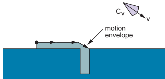
Figure 26.25 The second motion command and the envelope of possible motions. Even with error, we will eventually get into the hole.
