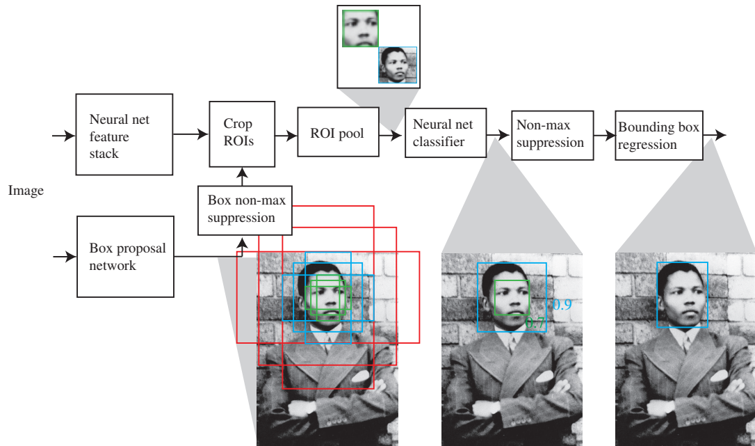
Figure 27.13 Faster RCNN uses two networks. A picture of a young Nelson Mandela is fed into the object detector. One network computes “objectness” scores of candidate image boxes, called “anchor boxes,” centered at a grid point. There are nine anchor boxes (three scales, three aspect ratios) at each grid point. For the example image, an inner green box and an outer blue box have passed the objectness test. The second network is a feature stack that computes a representation of the image suitable for classification. The boxes with highest objectness score are cut from the feature map, standardized in size with ROI pooling, and passed to a classifier. The blue box has a higher score than the green box and overlaps it, so the green box is rejected by non-maximum suppression. Finally, bounding box regression the blue box so that it fits the face. This means that the relatively coarse sampling of locations, scales, and aspect ratios does not weaken accuracy. Photo by Sipa/Shutterstock.
