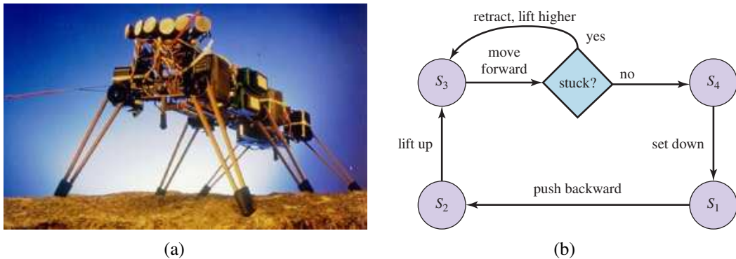
Figure 26.32 (a) Genghis, a hexapod robot. (Image courtesy of Rodney A. Brooks.) (b) An augmented finite state machine (AFSM) that controls one leg. The AFSM reacts to sensor feedback: if a leg is stuck during the forward swinging phase, it will be lifted increasingly higher.
