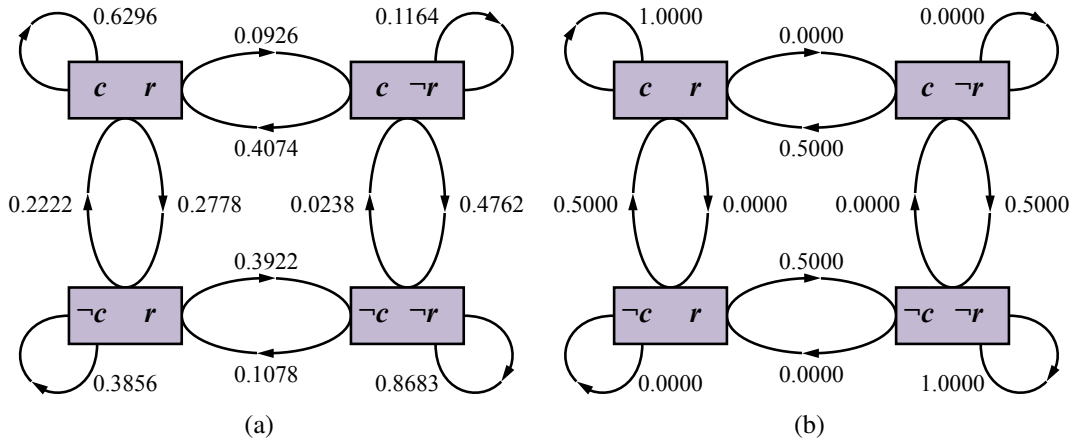
Figure 13.21 (a) The states and transition probabilities of the Markov chain for the query \mathbf{P}(\text{Rain} \mid \text{Sprinkler} = \text{true}, \text{WetGrass} = \text{true}) . Note the self-loops: the state stays the same when either variable is chosen and then resamples the same value it already has. (b) The transition probabilities when the CPT for Rain constrains it to have the same value as Cloudy .
