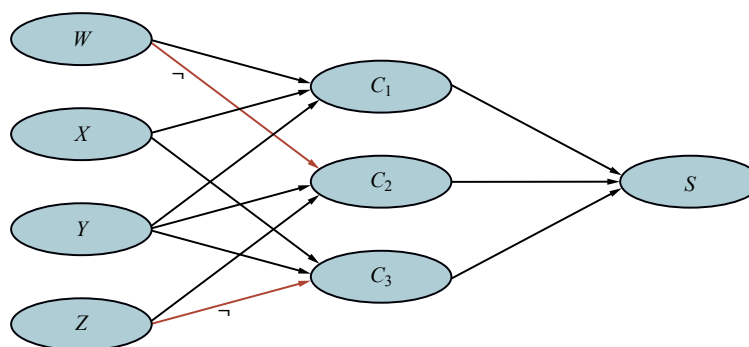
Figure 13.14 Bayes net encoding of the 3-CNF sentence
