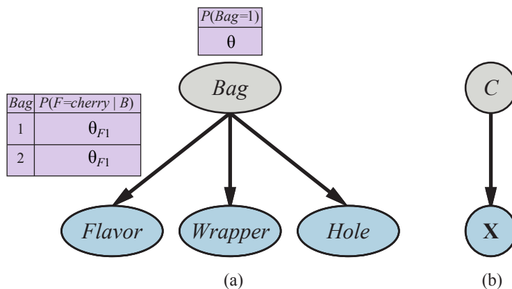
Figure 21.14 (a) A mixture model for candy. The proportions of different flavors, wrappers, and presence of holes depend on the bag, which is not observed. (b) Bayesian network for a Gaussian mixture. The mean and covariance of the observable variables \mathbf{X} depend on the component C .
