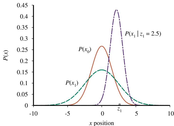
Figure 14.10 Stages in the Kalman filter update cycle for a random walk with a prior given by \mu_0=0.0 and \sigma_0=1.5 , transition noise given by \sigma_x=2.0 , sensor noise given by \sigma_z=1.0 , and a first observation z_1=2.5 (marked on the x -axis). Notice how the prediction P(x_1) is flattened out, relative to P(x_0) , by the transition noise. Notice also that the mean of the posterior distribution P(x_1 | z_1) is slightly to the left of the observation z_1 because the mean is a weighted average of the prediction and the observation.
