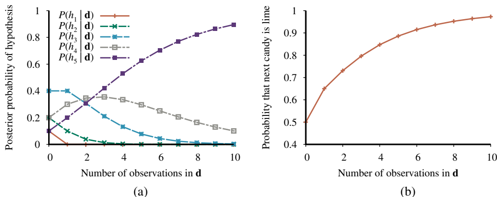
Figure 21.1 (a) Posterior probabilities P(h_i | d_1, \dots, d_N) from Equation (21.1). The number of observations N ranges from 1 to 10, and each observation is of a lime candy. (b) Bayesian prediction P(D_{N+1} = \text{lime} | d_1, \dots, d_N) from Equation (21.2).
