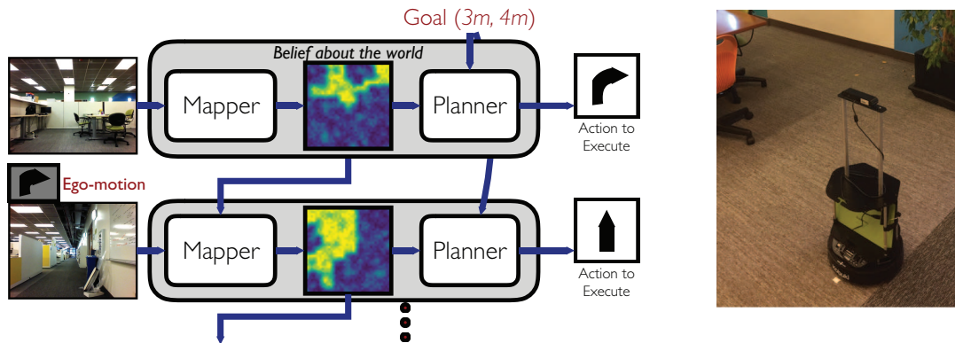
Figure 27.29 Navigation is tackled by decomposition into two problems: mapping and planning. With each successive time step, information from sensors is used to incrementally build an uncertain model of the world. This model along with the goal specification is passed to a planner that outputs the next action that the robot should take in order to achieve the goal. Models of the world can be purely geometric (as in classical SLAM), or semantic (as obtained via learning), or even topological (based on landmarks). The actual robot appears on the right. Figures courtesy of Saurabh Gupta.
