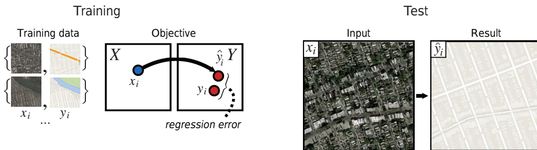
Figure 27.24 Paired image translation where the input consists of aerial images and the corresponding map tiles, and the goal is to train a network to produce a map tile from an aerial image. (The system can also learn to generate aerial images from map tiles.) The network is trained by comparing \hat{y}_i (the output for example x_i of type X ) to the right output y_i of type Y . Then at test time, the network must make new images of type Y from new inputs of type X . Figure courtesy of Phillip Isola, Jun-Yan Zhu and Alexei A. Efros, produced by a system described in Isola et al. (2017). Map data © 2019 Google.
