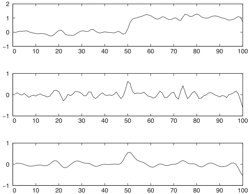
Figure 27.7 Top: Intensity profile I(x) along a one-dimensional section across a step edge. Middle: The derivative of intensity, I'(x) . Large values of this function correspond to edges, but the function is noisy. Bottom: The derivative of a smoothed version of the intensity. The noisy candidate edge at x = 75 has disappeared.
