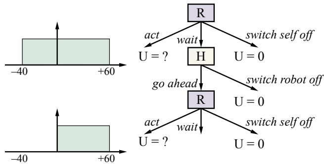
Figure 15.11 The off-switch game. R , the robot, can choose to act now, with a highly uncertain payoff; to switch itself off; or to defer to H , the human. H can switch R off or let it go ahead. R now has the same choice again. Acting still has an uncertain payoff, but now R knows the payoff is nonnegative.
