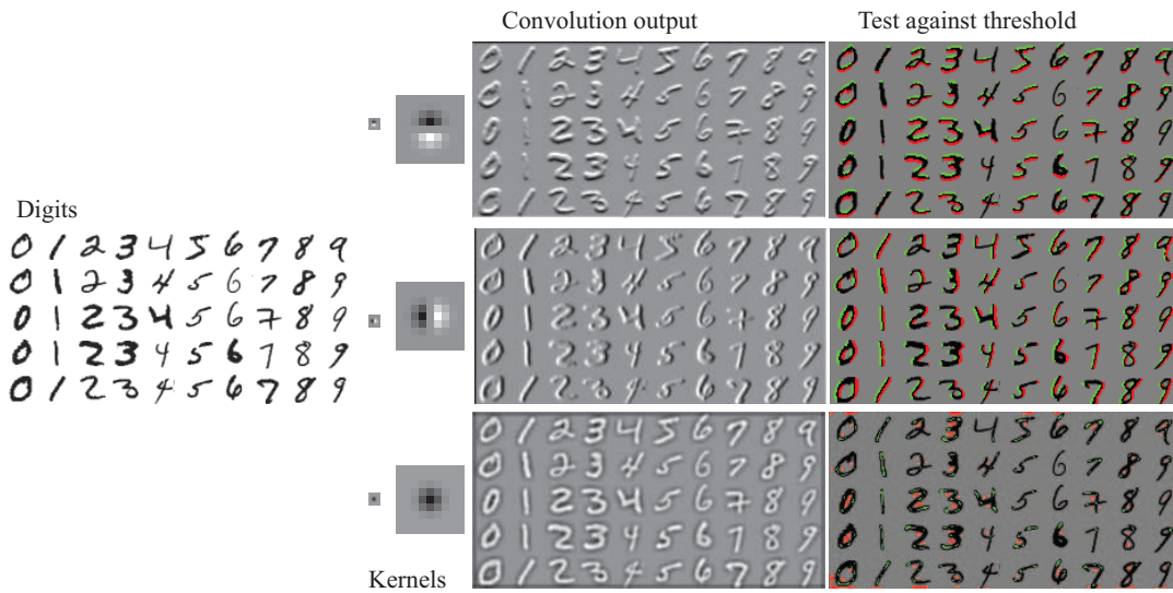
Figure 27.12 On the far left, some images from the MNIST data set. Three kernels appear on the center left. They are shown at actual size (tiny blocks) and magnified to reveal their content: mid-grey is zero, light is positive, and dark is negative. Center right shows the results of applying these kernels to the images. Right shows pixels where the response is bigger than a threshold (green) or smaller than a threshold (red). You should notice that this gives (from top to bottom): a horizontal bar detector; a vertical bar detector; and (harder to note) a line ending detector. These detectors pay attention to the contrast of the bar, so (for example) a horizontal bar that is light on top and dark below produces a positive (green) response, and one that is dark on top and light below gets a negative (red) response. These detectors are moderately effective, but not perfect.
