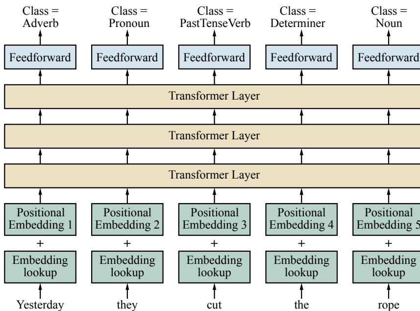
Figure 25.10 Using the transformer architecture for POS tagging.
