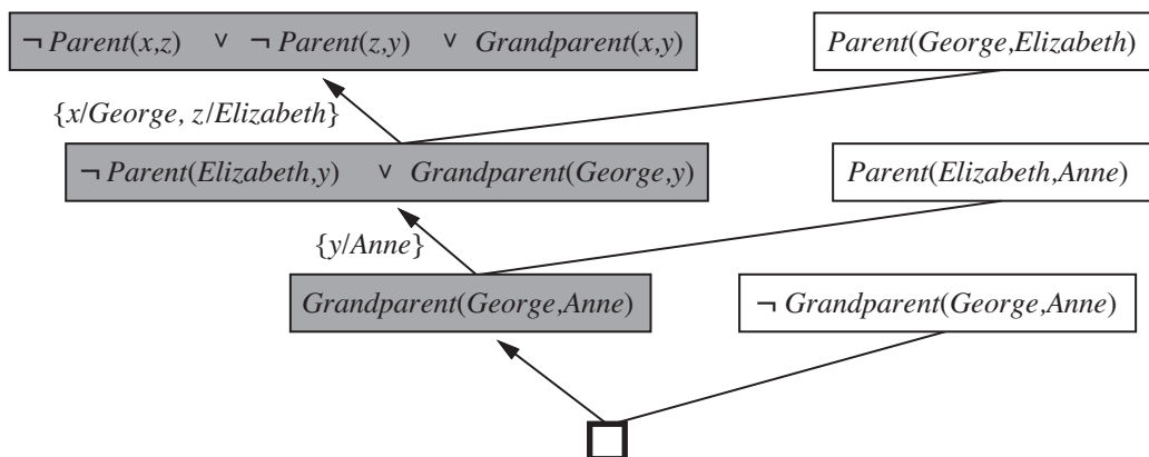
Figure 20.13 Early steps in an inverse resolution process. The shaded clauses are generated by inverse resolution steps from the clause to the right and the clause below. The unshaded clauses are from the Descriptions and Classifications (including negated Classifications ).
