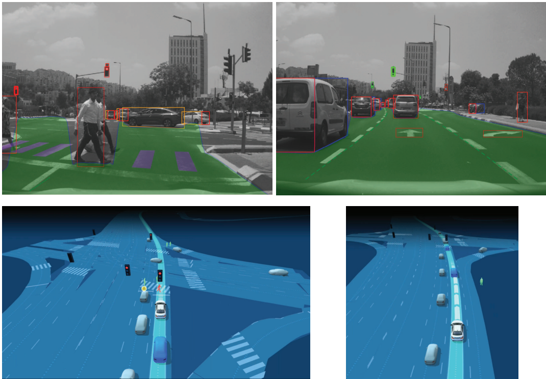
Figure 27.28 Mobileye’s camera-based sensing for autonomous vehicles. Top row: Two images from a front-facing camera, taken a few seconds apart. The green area is the free space—the area to which the vehicle could physically move in the immediate future. Objects are displayed with 3D bounding boxes defining their sides (red for the rear, blue for the right side, yellow for the left side, and green for the front). Objects include vehicles, pedestrians, the inner edge of the self-lane marks (necessary for lateral control), other painted road and crosswalk marks, traffic signs, and traffic lights. Not shown are animals, poles and cones, sidewalks, railings, and general objects (e.g., a couch that fell from the back of a truck). Each object is then marked with a 3D position and velocity. Bottom row: A full physical model of the environment, rendered from the detected objects. (Images show Mobileye’s vision-only system results). Images courtesy of Mobileye.
