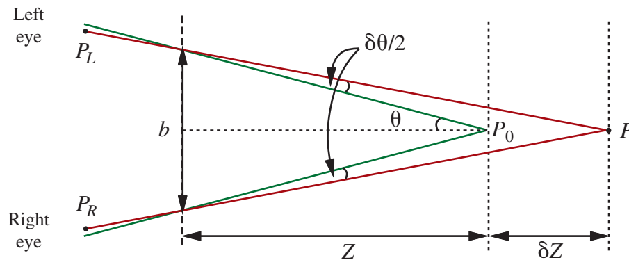
Figure 27.15 The relation between disparity and depth in stereopsis. The centers of projection of the two eyes are distance b apart, and the optical axes intersect at the fixation point P_0 . The point P in the scene projects to points P_L and P_R in the two eyes. In angular terms, the disparity between these is \delta\theta (the diagram shows two angles of \delta\theta/2 ).
