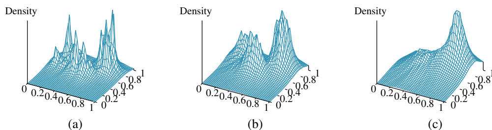
Figure 21.9 Density estimation using k -nearest-neighbors, applied to the data in Figure 21.8(b), for k=3 , 10, and 40 respectively. k=3 is too spiky, 40 is too smooth, and 10 is just about right. The best value for k can be chosen by cross-validation.
