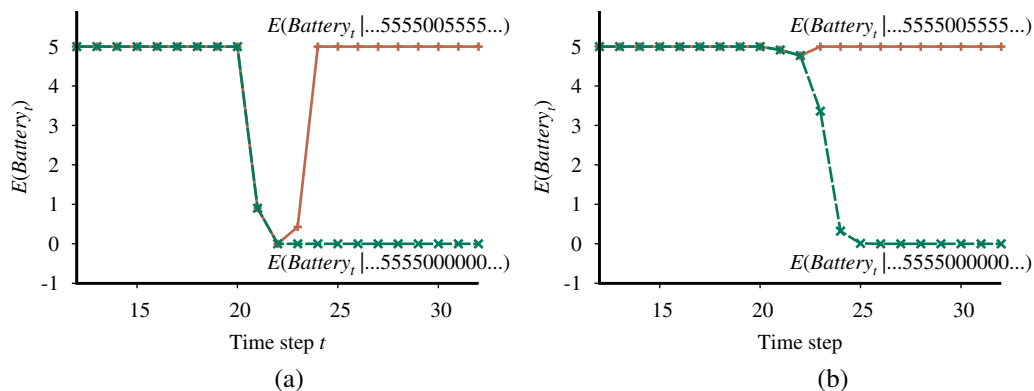
Figure 14.14 (a) Upper curve: trajectory of the expected value of \text{Battery}_t for an observation sequence consisting of all 5s except for 0s at t=21 and t=22 , using a simple Gaussian error model. Lower curve: trajectory when the observation remains at 0 from t=21 onwards. (b) The same experiment run with the transient failure model. The transient failure is handled well, but the persistent failure results in excessive pessimism about the battery charge.
