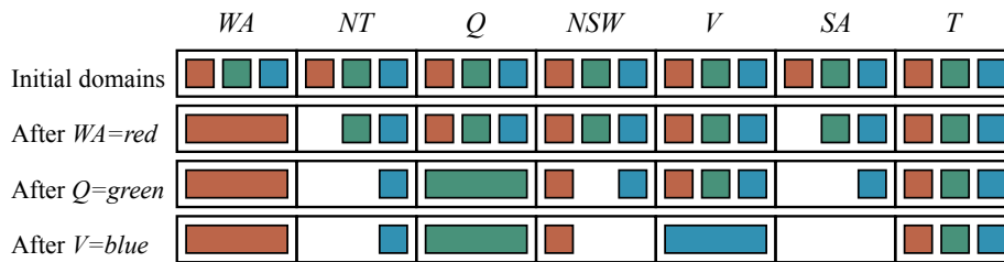
Figure 5.7 The progress of a map-coloring search with forward checking. WA=red is assigned first; then forward checking deletes red from the domains of the neighboring variables NT and SA . After Q=green is assigned, green is deleted from the domains of NT , SA , and NSW . After V=blue is assigned, blue is deleted from the domains of NSW and SA , leaving SA with no legal values.
