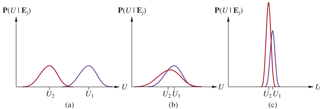
Figure 15.8 Three generic cases for the value of information. In (a), a_1 will almost certainly remain superior to a_2 , so the information is not needed. In (b), the choice is unclear and the information is crucial. In (c), the choice is unclear, but because it makes little difference, the information is less valuable. (Note: The fact that U_2 has a high peak in (c) means that its expected value is known with higher certainty than U_1 .)
