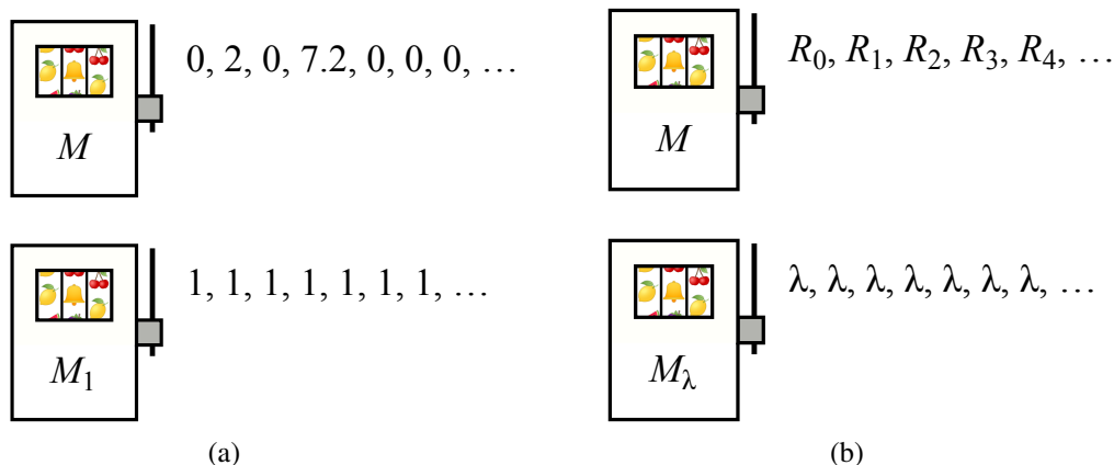
Figure 16.12 (a) A simple deterministic bandit problem with two arms. The arms can be pulled in any order, and each yields the sequence of rewards shown. (b) A more general case of the bandit in (a), where the first arm gives an arbitrary sequence of rewards and the second arm gives a fixed reward \lambda .
