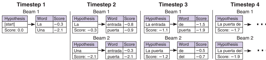
Figure 25.8 Beam search with beam size of b=2 . The score of each word is the log-probability generated by the target RNN softmax, and the score of each hypothesis is the sum of the word scores. At timestep 3, the highest scoring hypothesis La entrada can only generate low-probability continuations, so it “falls off the beam.”
