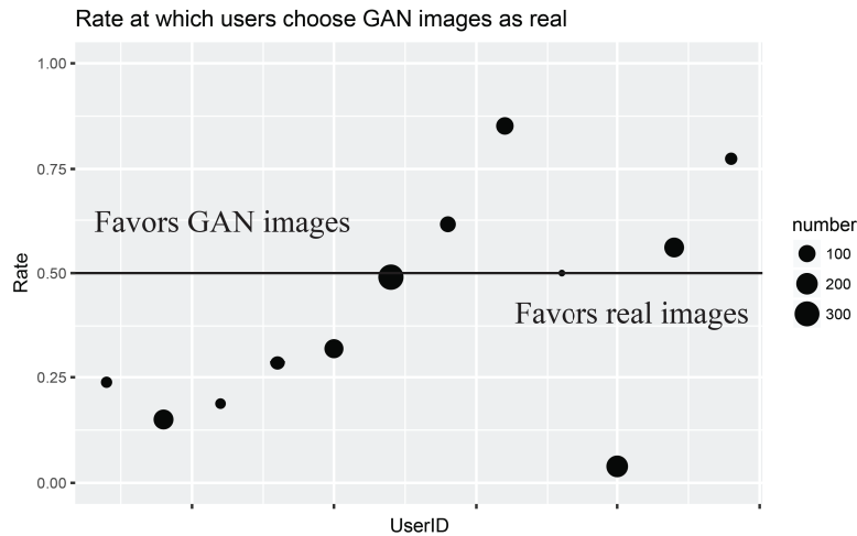
Figure 27.27 GAN generated images of lung X-rays. On the left, a pair consisting of a real X-ray and a GAN-generated X-ray. On the right, results of a test asking radiologists, given a pair of X-rays as seen on the left, to tell which is the real X-ray. On average, they chose correctly 61% of the time, somewhat better than chance. But they differed in their accuracy—the chart on the right shows the error rate for 12 different radiologists; one of them had an error rate near 0% and another had 80% errors. The size of each dot indicates the number of images each radiologist viewed. Figure courtesy of Alex Schwing, produced by a system described in Deshpande et al. (2019).
